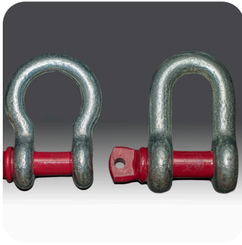
D Shackles & Bow Shackles
